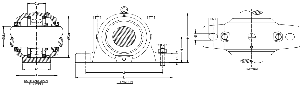
Plummer Blocks ( Bearing housings ) Series SNA 500 for bearings with adapter sleeves.
