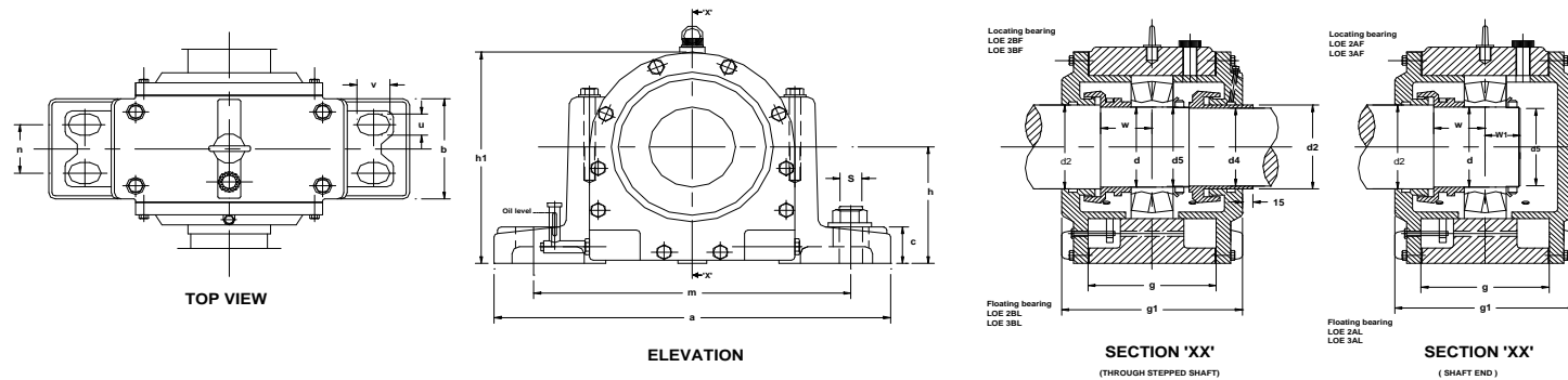
Bearing Housing (Plummer Block) of Series LOE-200&300 Suitable for Spherical Roller Bearing with Cylindrical Bore.
