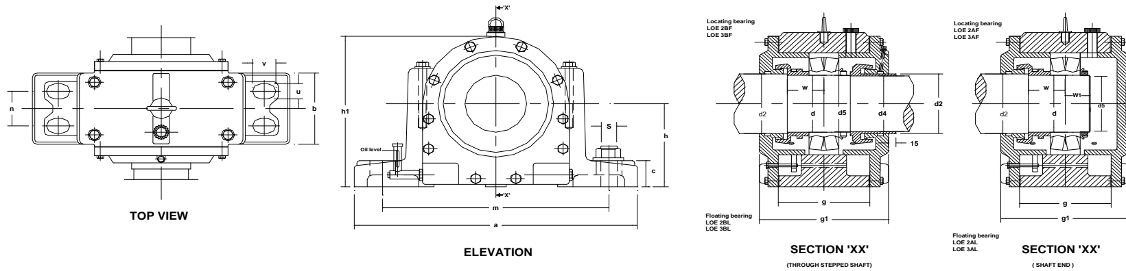
Bearing Housing (Plummer Block) of Series LOE-500&600 Suitable for Spherical Roller Bearing with Adapter Sleeve.
