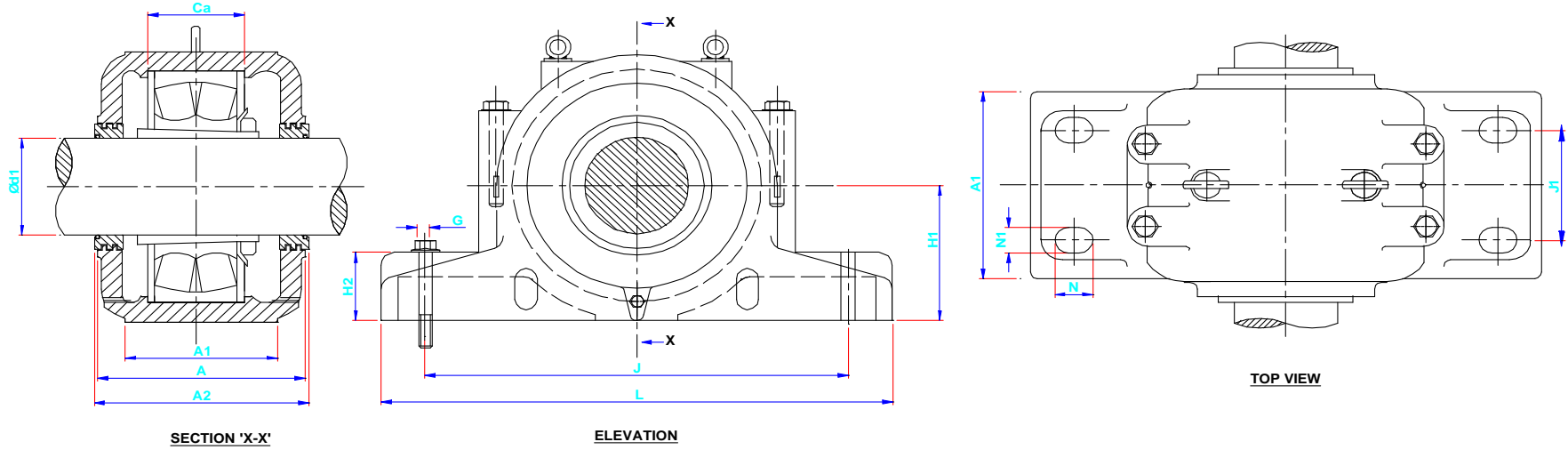
Masta Plummer block Series SD 33 Suitable for bearing Series 230K
