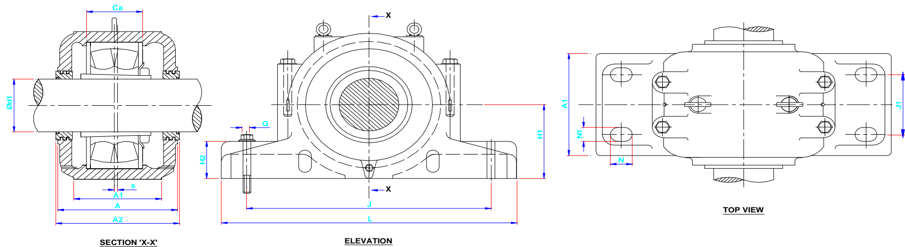
Masta Brand SD Series Plummer Block with Labyrinth collars For bearing with tapered boer and adapter sleeves
