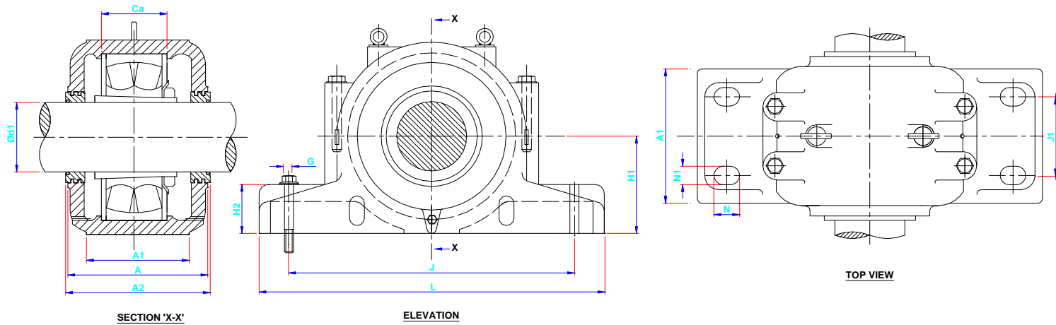
Masta Brand SD 30 Series Plummer Block with Labyrinth collars For bearing with tapered bore and adapter sleeves.
