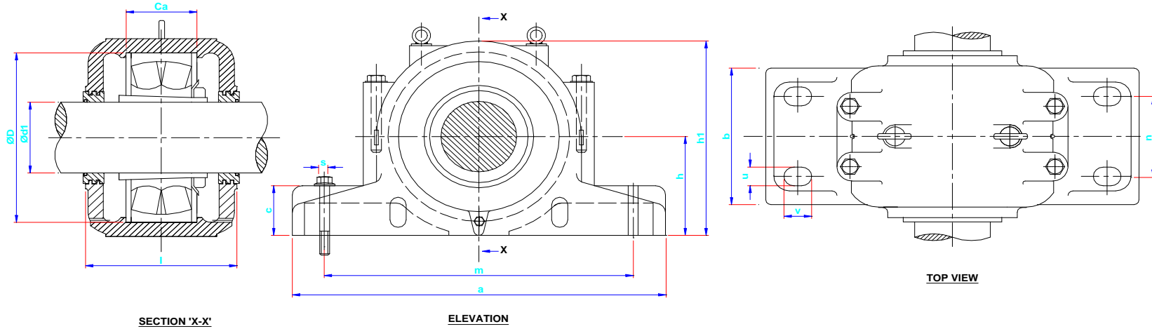
Masta Brand SD 500 Series Plummer Block with felt Seals For bearing with tapered bore and adapter sleeves.
