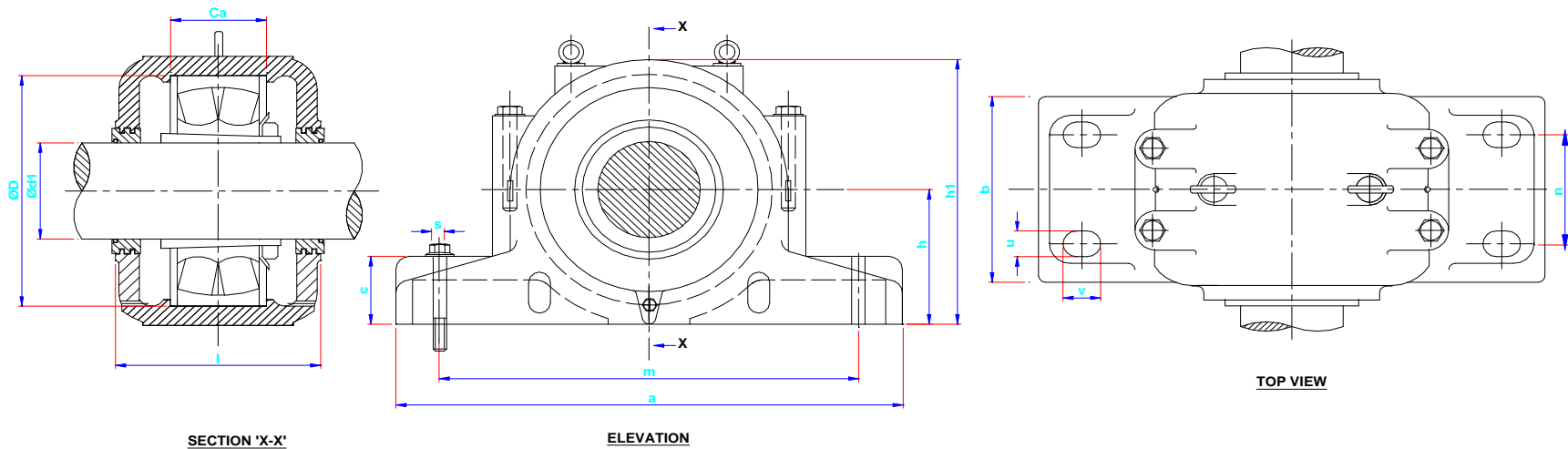
Masta Brand SD 600 Series Plummer Block with felt seals For bearing with tapered bore and adapter sleeves.
