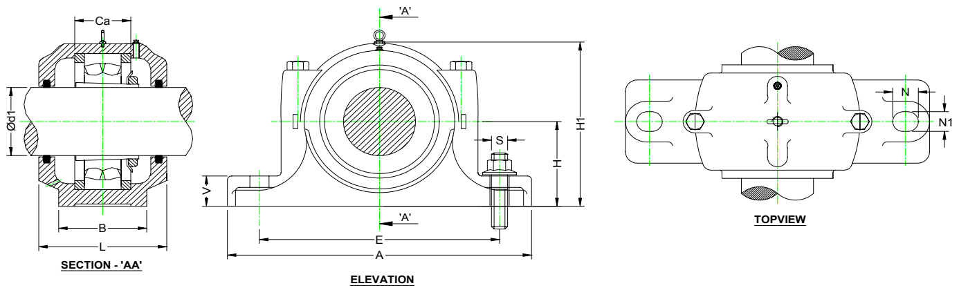
Plummer Blocks ( Bearing housings ) Series SN 500 for bearings with adapter sleeves.
