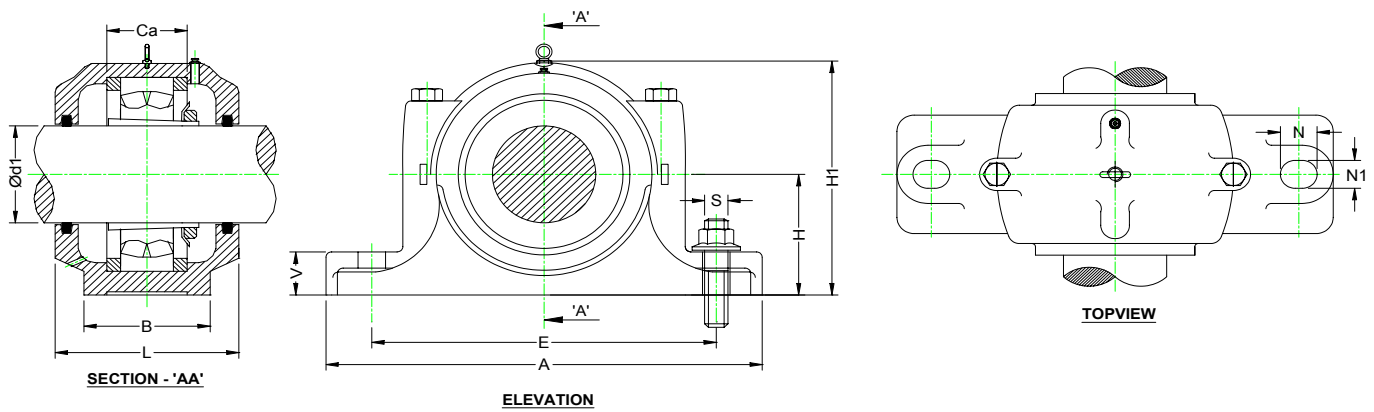
Plummer Blocks ( Bearing housings ) Series SN 600 for bearings with adapter sleeves.
