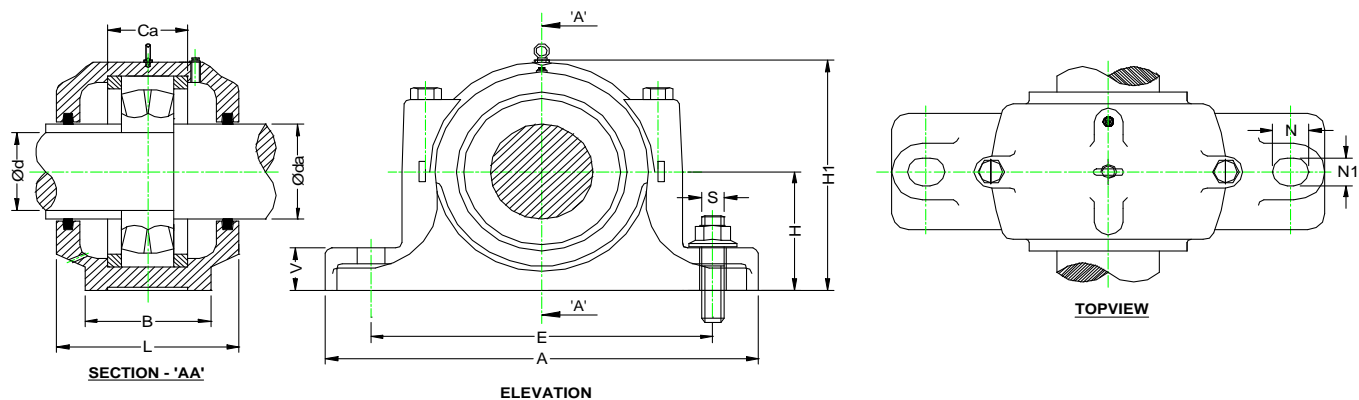
Plummer Blocks ( Bearing housings ) Series SN 200 for bearings with Cylindrical Bore
