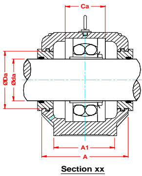
Plummer Blocks ( Bearing housings ) SNH Series 500 for bearings with adapter sleeves.
