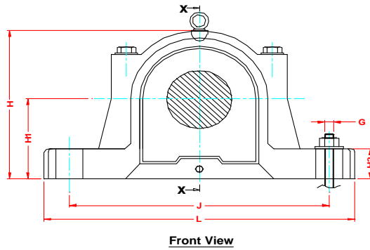
Plummer Blocks ( Bearing housings ) SNH Series 500 for bearings with adapter sleeves.
