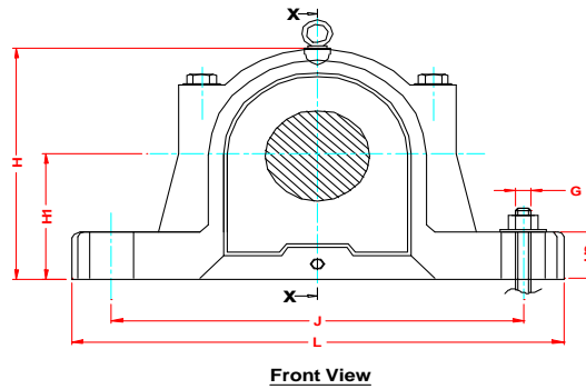
Plummer Blocks ( Bearing housings ) Series SNH 500 for bearings with adapter sleeves.
