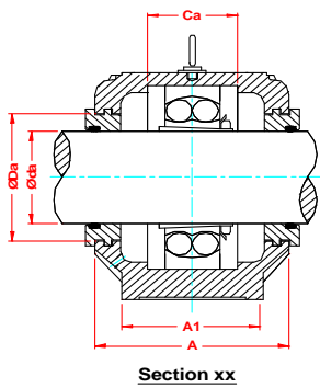
Plummer Blocks ( Bearing housings ) Series SNH 500 for bearings with adapter sleeves.
