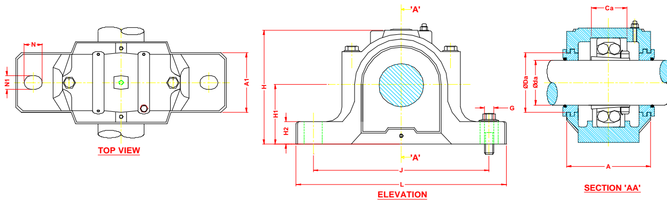
MASTA SNL PLUMMER BLOCK HOUSING FOR BEARINGS WITH ADAPTER SLEEVES
