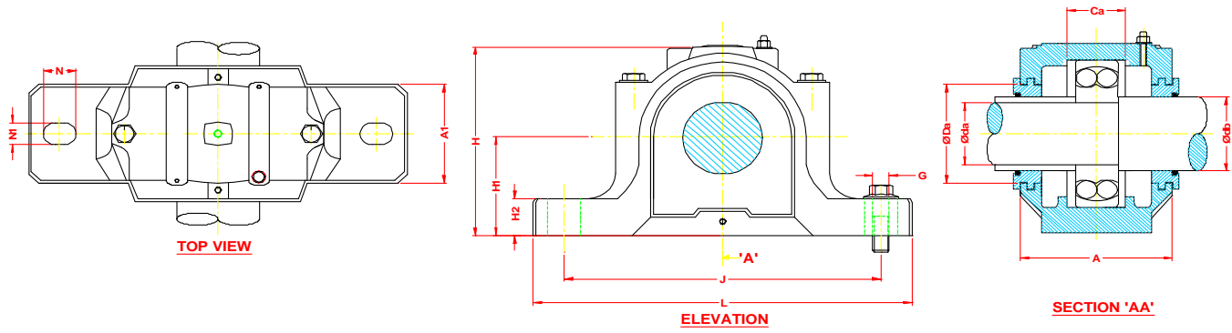
MASTA SNL PLUMMER BLOCK HOUSING FOR STRAIGHT (CYLINDRICAL) BORE BEARINGS
