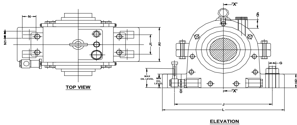
SOFN Plummer Block for spherical roller bearing with Adapter Sleeve (FOR DIRECT MOUNTING )
